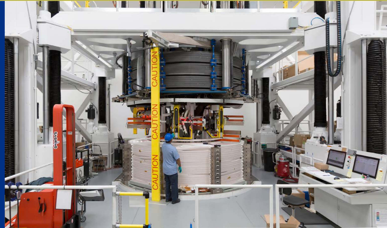
Turn insulation station structure lifts and raises 110-tonne module and releases individual turns for insulation wrapping
