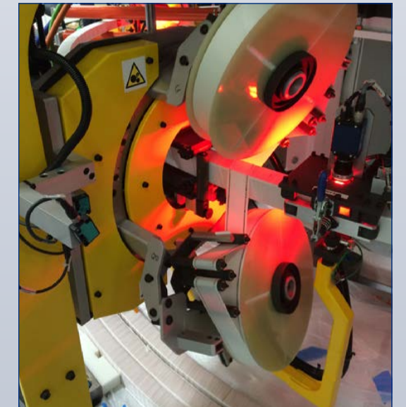
Automated heads wrapping fiberglass tape around the conductor
